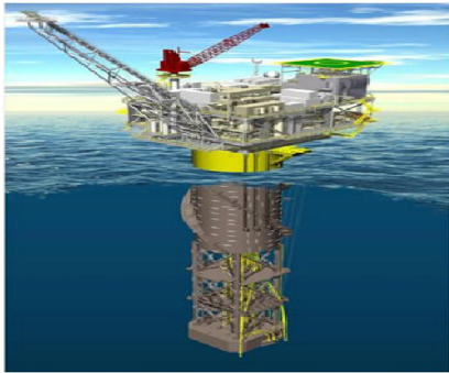
Figure 5: Spar
